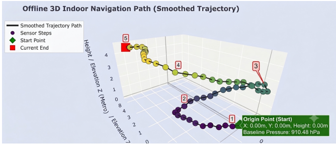
Fig. 2. Reconstructed 3D indoor multi-floor walking trajectory generated on the i.MX RT1064. The trajectory highlights critical spatial waypoints, including the origin ( Z = 0.00 m, P_0 = 910.48 hPa), stair ascension, landing turn, and arrival at the 1st floor destination.
